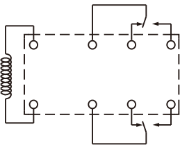
Wiring diagram (bottom view) 接线图 (底视图)
